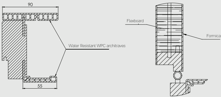
Carved hardwood door frame with WPC Architraves
