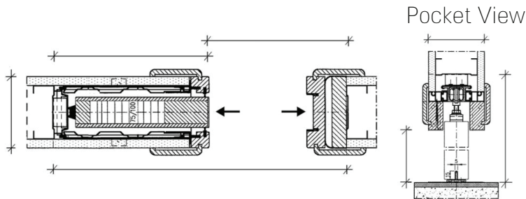
POCKET SLIDING DOORS SPECIFICATION
